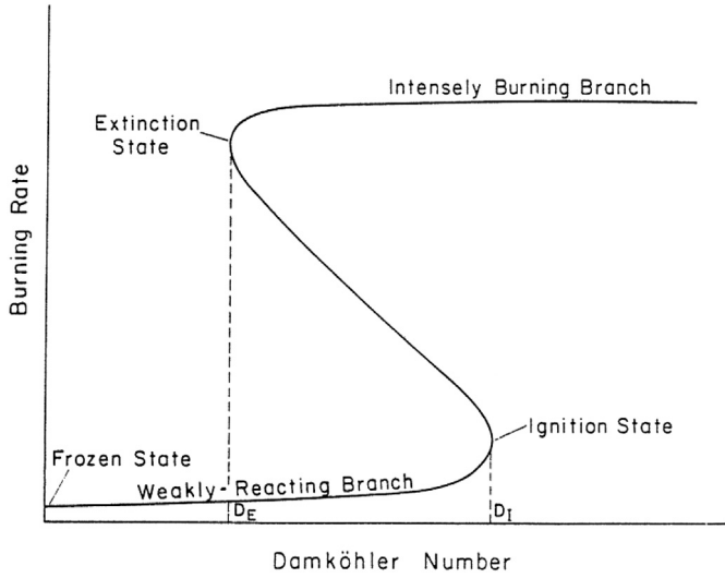
Fig. 2. Characteristic S-curve showing all possible modes of droplet gasification, including pure vaporization ( D = 0 ), ignition ( D = D_I ), pure combustion ( D = \infty ) and extinction ( D = D_E ). From Ref. [19].
