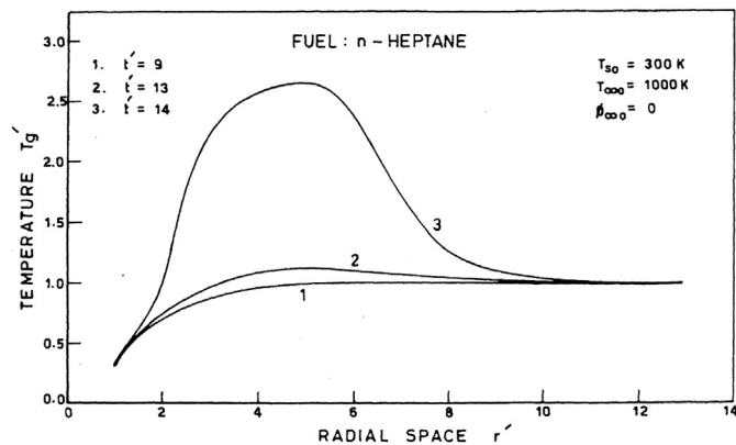
Fig. 18. Predicted gas temperature profiles at different times before and at the instant of ignition for n-heptane fuel droplet in air at a temperature of 1000 K. From Ref. [50].
