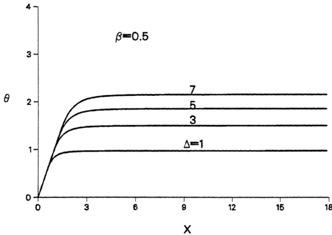
Fig. 3. Variation of the perturbed temperature in the reaction zone as a function of the stretched variable for \beta = 0.5 and different Damköhler numbers. From Ref. [21].
