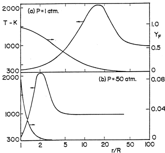
Fig. 34. Radial profiles of gas temperature and fuel vapor mass fraction at the time of ignition for two different pressures. From Ref. [47].
