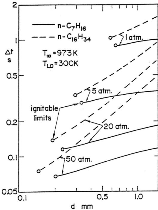
Fig. 33. Predicted ignition delay time as a function of droplet diameter for n-heptane and n-hexadecane droplets for different ambient pressures. The ambient gas temperature is 973 K. From Ref. [46].
