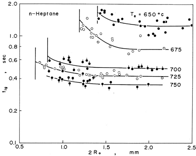
Fig. 10. Measured ignition delay time versus droplet diameter for n-heptane droplets for different ambient gas temperatures. From Ref. [26].
