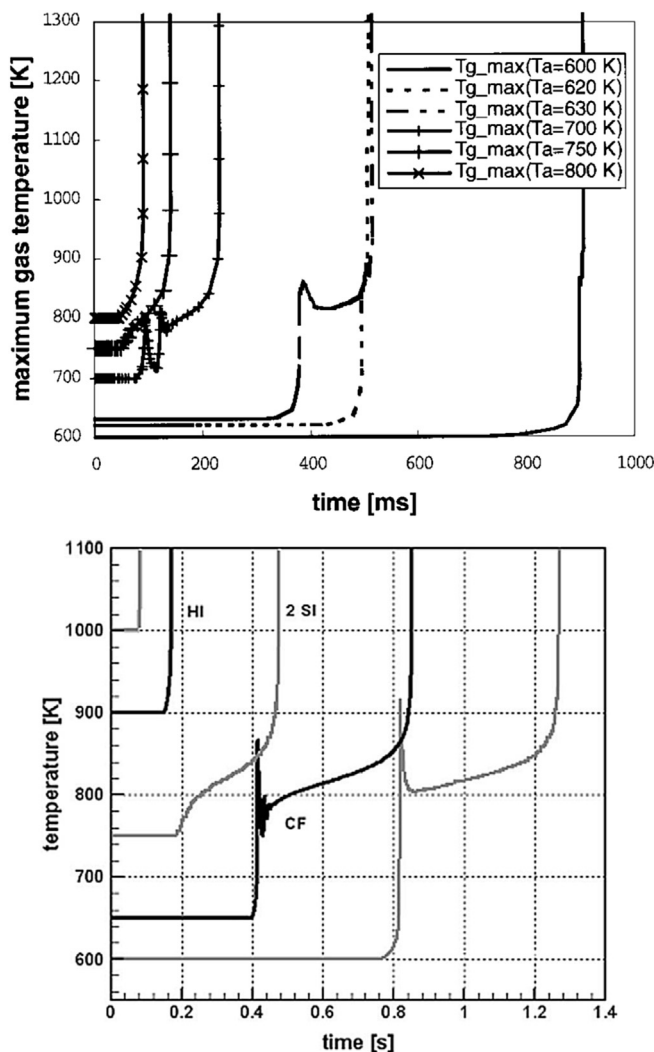
Fig. 27. Various ignition regimes shown in terms of the temporal evolution of the maximum gas temperature. Top figure from Schnaubelt et al. [47] is for n-heptane droplet, while the bottom figure from Cuoci et al. [48] is for n-decane droplet.
