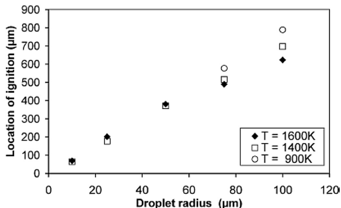
Fig. 30. Ignition location plotted with respect to initial droplet radius. From Ref. [59].
