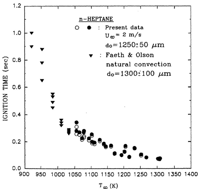
Fig. 42. Measured ignition delay time versus ambient temperature for n-heptane droplets in forced and natural convection. From Ref. [72].
