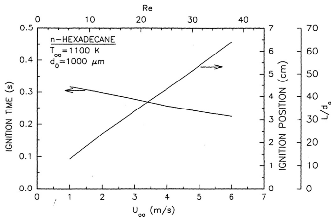
Fig. 45. The effect of free stream velocity on the computed ignition delay times and ignition locations. From Ref. [73].
