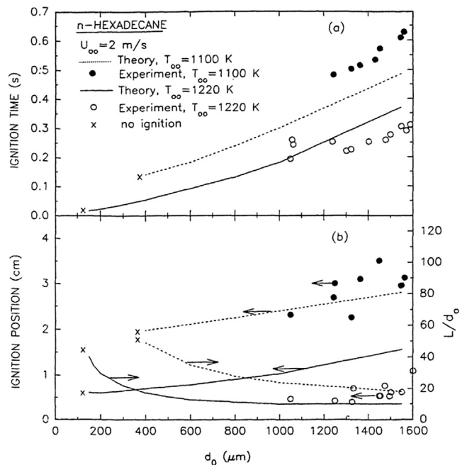
Fig. 44. The computed and measured ignition delay time (a) and ignition location (b) plotted versus initial droplet diameter for n-hexadecane droplets. From Ref. [73].
