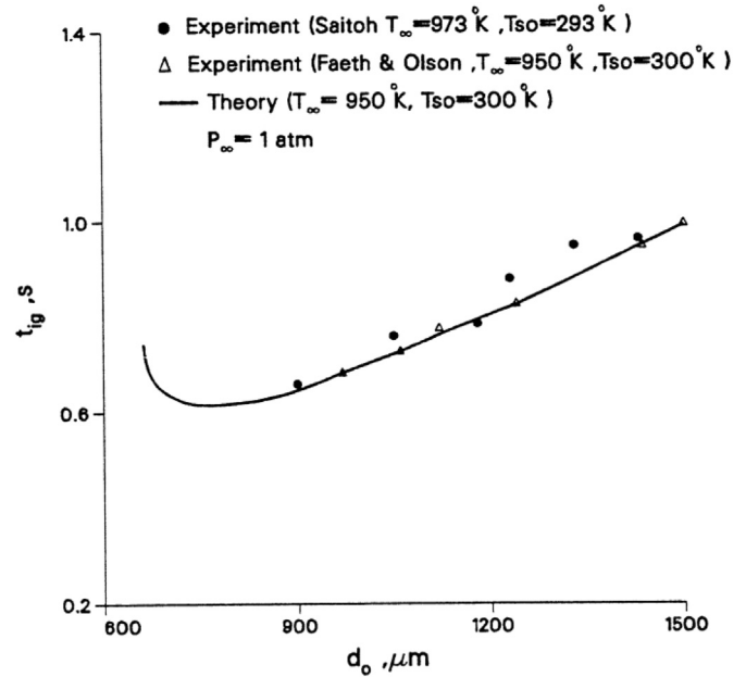
Fig. 6. Computed and measured ignition delays plotted as a function of the initial drop size for n-hexadecane droplets. From Ref. [21].
