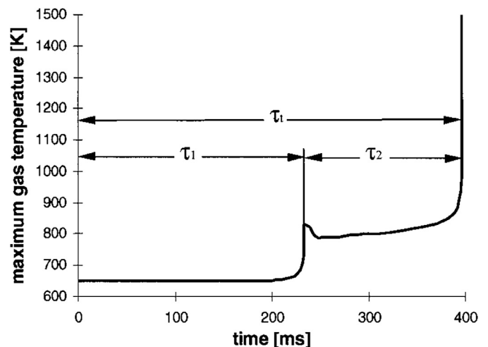
Fig. 14. Two-stage ignition process for a n-heptane droplet illustrated by the temporal variation of the peak gas temperature. The droplet diameter = 0.7 mm, T_a = 650 K, and p = 5 atm. The first ( \tau_1 ), second ( \tau_2 ), and total ignition times are indicated. From Ref. [47].
