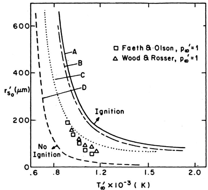
Fig. 8. Computed and measured ignition limits for n-hexadecane droplets. Curve A: C_{pl} = 0.69 cal/gm/K, p = 1 atm, B: C_{pl} = 0.52 cal/gm/K, p = 1 atm, C: Same as curve A but activation energy reduced by 12 percent, D: C_{pl} = 0.69 cal/gm/K, p = 10 atm. From Ref. [27].
