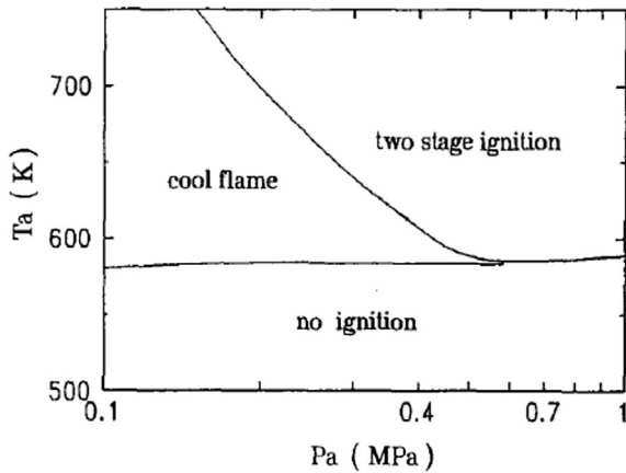
Fig. 15. Various ignition regions mapped in terms of ambient temperature and pressure under normal-gravity conditions. From Ref. [39].
