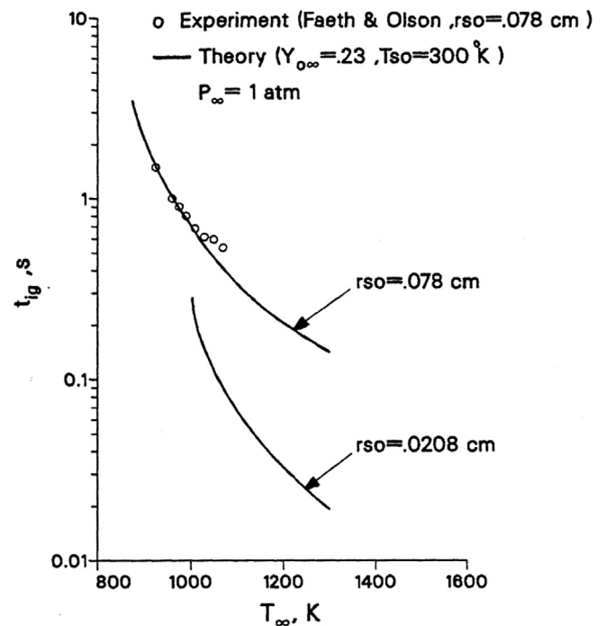
Fig. 7. Computed and measured ignition delays plotted versus ambient temperature for n-hexadecane droplets. From Ref. [21].
