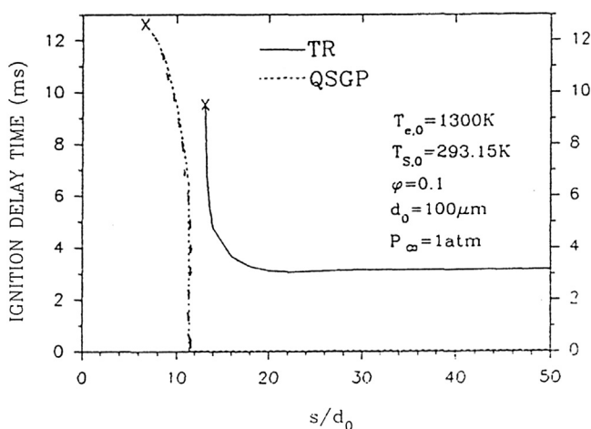
Fig. 23. Comparison of ignition delays versus inter-droplet spacing obtained by using the quasi-steady and transient gas-phase models for n-heptane droplets. Here TR and QSGP refer to the transient and quasi-steady models respectively. From Ref. [52].
