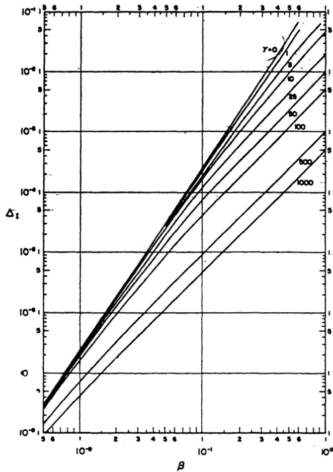
Fig. 9. Ignition Damköhler number as function of heat transfer parameter ( \beta ) and fuel concentration parameter ( \gamma ). From Ref. [30].
