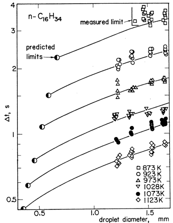
Fig. 12. Predicted and measured ignition delay times for n-hexadecane droplets as a function of droplet diameter. From Ref. [38].
