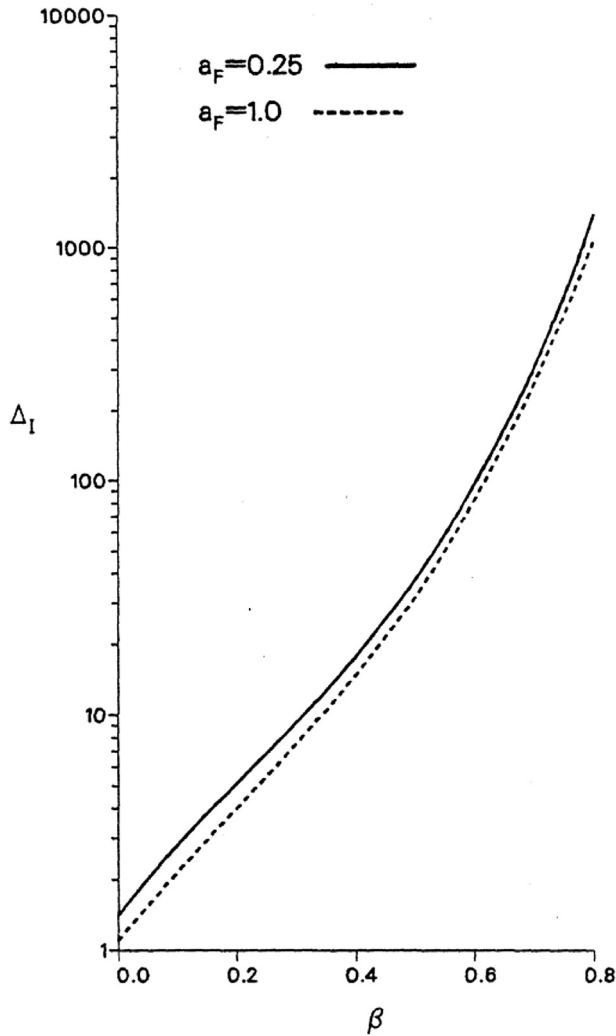
Fig. 5. Variation of ignition Damköhler number with \beta . From Ref. [21].
