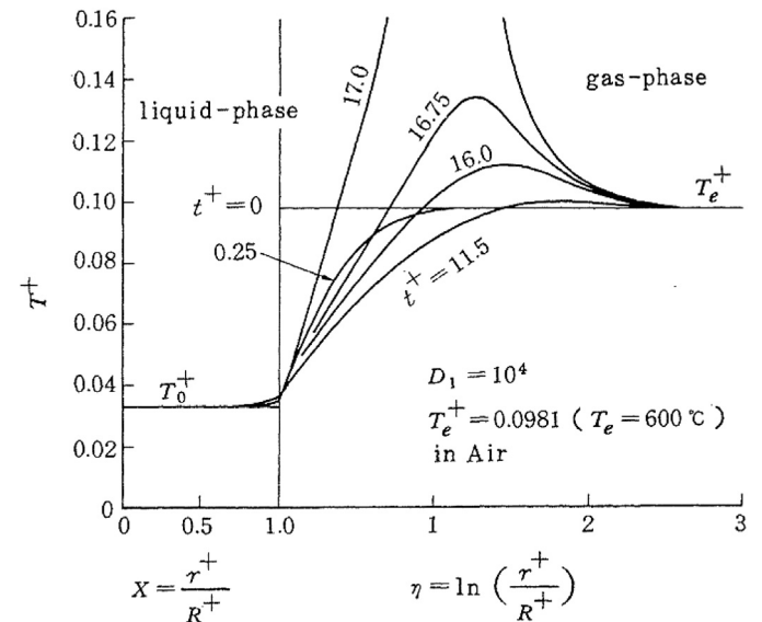
Fig. 17. Temporal history of the (nondimensional) radial temperature profiles showing the ignition event. From Ref. [49].
