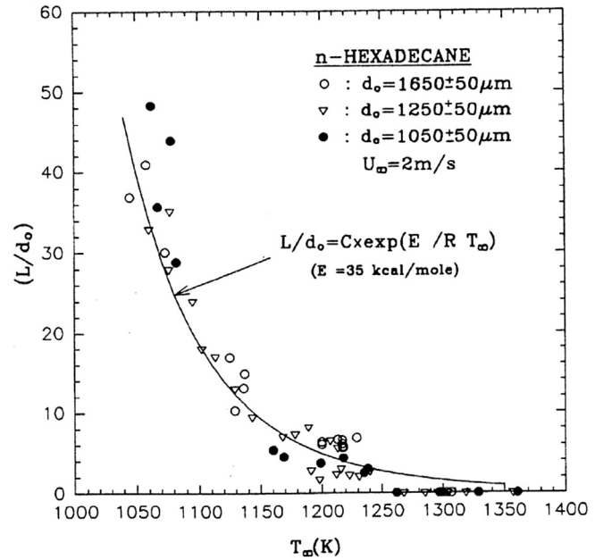
Fig. 40. Normalized ignition location in the droplet wake plotted as a function of ambient temperature for different initial diameters. From Ref. [72].
