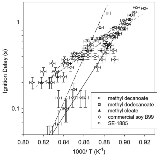
Fig. 37. Normal-gravity ignition delay versus ambient temperature for 1.2 mm droplets of methyl decanoate, methyl dodecanoate, methyl oleate, SE-1885 soy methyl ester and commercial B99 soy methyl ester. Pressure is 1 atm. From Ref. [43].
