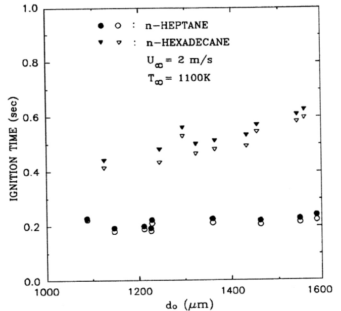
Fig. 41. Measured ignition delay time versus initial diameter for n-heptane and n-hexadecane droplets. The open and filled symbols respectively indicate the times when ignition occurs and when an envelope flame forms. From Ref. [72].
