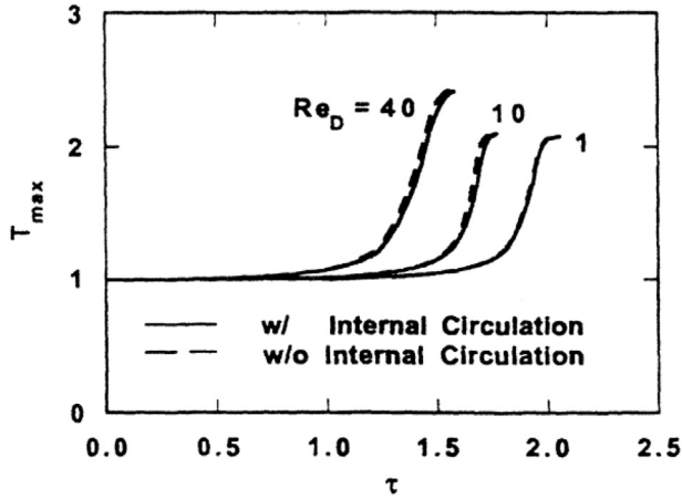
Fig. 38. Temporal variation of the maximum gas temperature for three different droplet Reynolds numbers. Here time is normalized by the momentum diffusion time, \tau = t\mu_{\infty}/a_0^2\rho_{\infty} . From Ref. [71].
