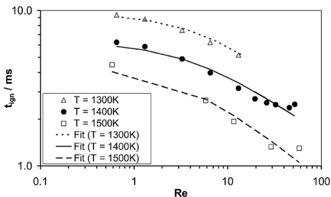
Fig. 46. Computed ignition delay time for a methanol droplet plotted versus the Reynolds number ( p = 7 bar, d_0 = 400 \mu\text{m} ). From Ref. [74].
