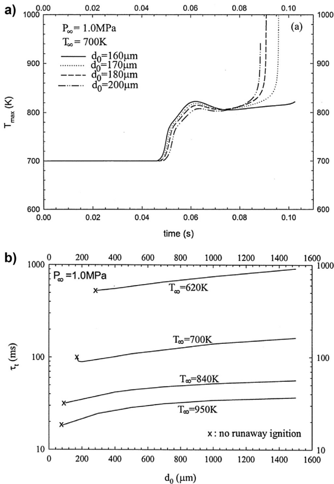
Fig. 28. (a) Temporal evolution of peak gas temperature for different droplet diameters (top). (b) Ignition delay plotted versus initial diameter for different ambient temperatures. From Ref. [60].
