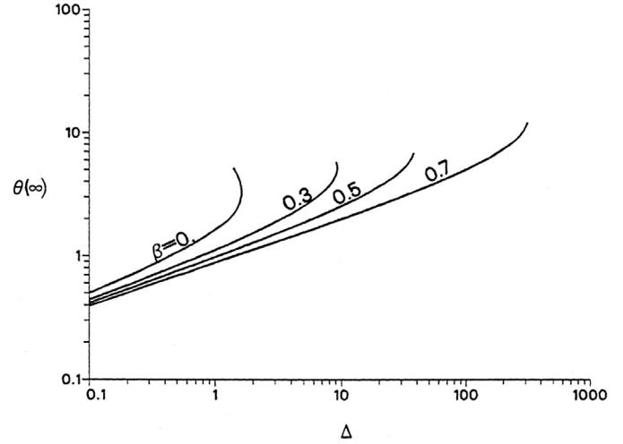
Fig. 4. Maximum perturbed temperature (corresponding to X \rightarrow \infty in Fig. 3) versus D for different values of \beta . From Ref. [21].
