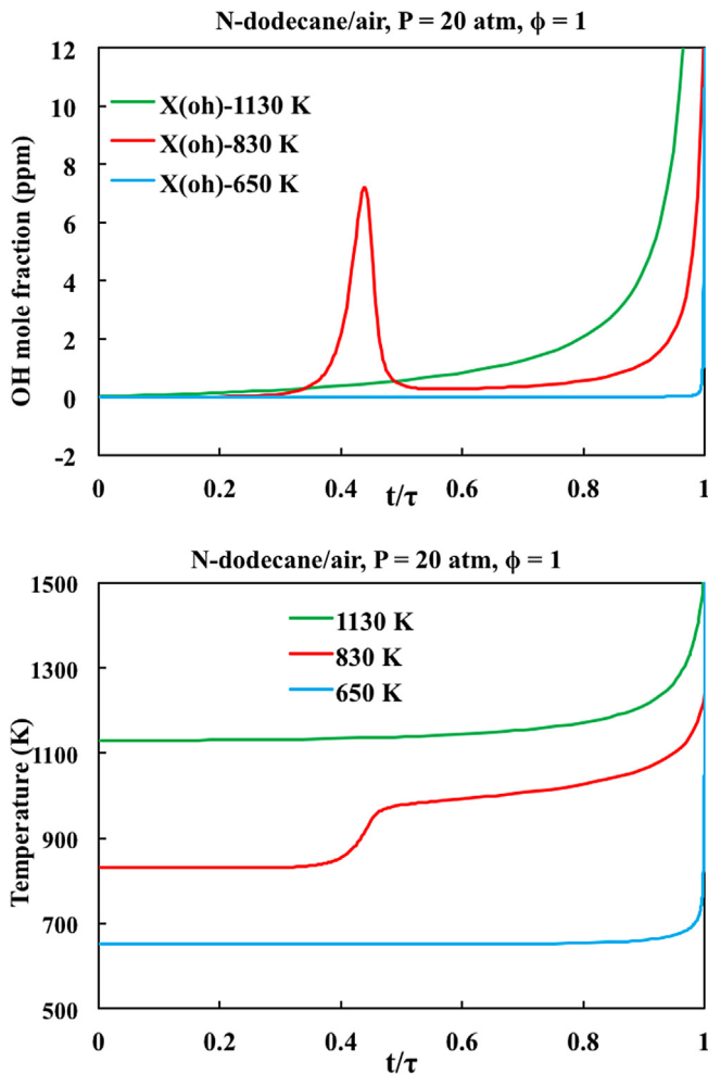
Fig. 25. Temporal variation of OH mole fraction and temperature for the ignition of homogeneous n-dodecane/air mixture for three different initial temperatures. Two-stage ignition is clearly indicated for the 830 K case. Here \tau is the ignition delay time.
