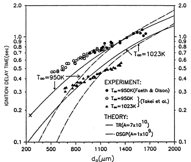
Fig. 22. Comparison of the measured and computed ignition delays using the QSDI and transient models. Here QSGP and TR denote quasi-steady gas phase, and transient models, respectively. From Ref. [51].
