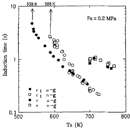
Fig. 16. Comparison of ignition delays plotted as a function of ambient temperature under normal and microgravity conditions. Solid symbols: \mu\text{g} data and open symbols: 1 g data. From Ref. [40].
