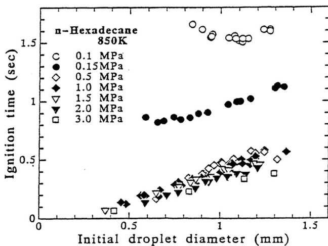
Fig. 31. Measured ignition delay versus initial droplet diameter for different pressures. Fiber-suspended n-hexadecane droplet in an electric furnace. From Ref. [67].
