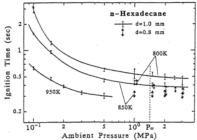
Fig. 32. Measured ignition delay versus pressure for fiber-suspended n-hexadecane droplets in an electric furnace. From Ref. [67].
