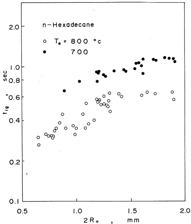
Fig. 11. Measured ignition delay time versus droplet diameter for n-hexadecane droplets for two different ambient temperatures. From Ref. [26].
