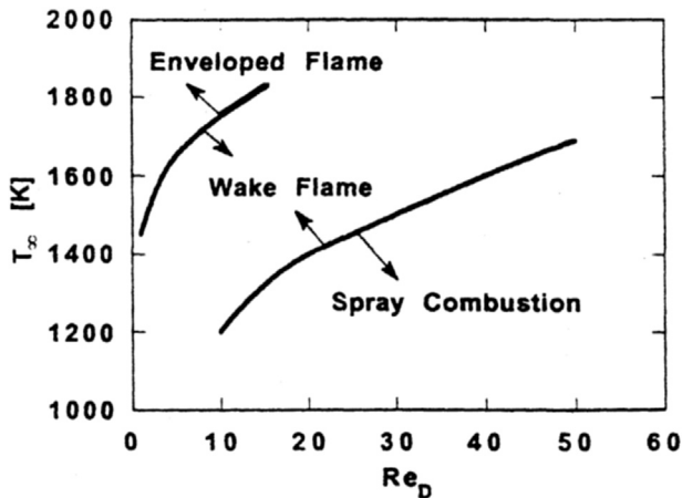
Fig. 39. Three flame regimes represented in ambient temperature–Reynolds number space. From Ref. [71].
