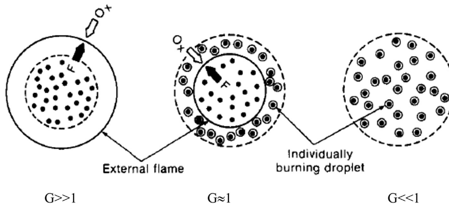
Fig. 47. A schematic of droplet/spray combustion regimes in terms of the non-dimensional Group number. From Ref. [75].
