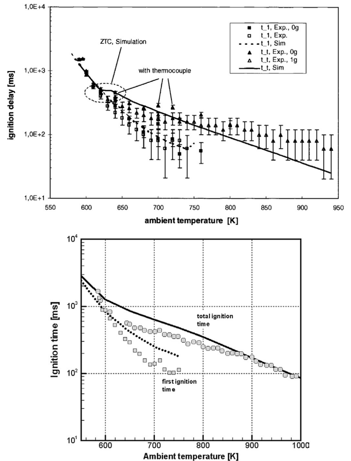
Fig. 29. Comparison of predicted and measured first and total ignition times. Droplet diameter is 0.7 mm. Top figure from Schnaubelt et al. [47] is for n-heptane at p = 5 \text{ atm} , and bottom figure from Couci et al. [48] for n-decane at p = 3 \text{ atm} .
