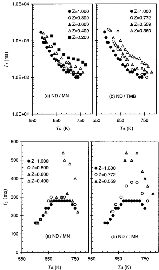
Fig. 36. Measured first-ignition (top) and second-ignition delay times versus ambient temperature for different compositions of ND/MN and ND/TMB blends. Droplet diameter is 0.7 mm and pressure is 3 atm. Parameter Z represents the fraction of n-decane in the blend.
