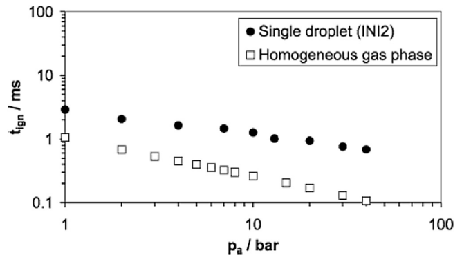
Fig. 35. Ignition delays for homogeneous n-heptane/air mixture and for droplets (initial diameter = 100 \mu m) plotted versus pressure for T_a = 1200 K. From Ref. [59].
