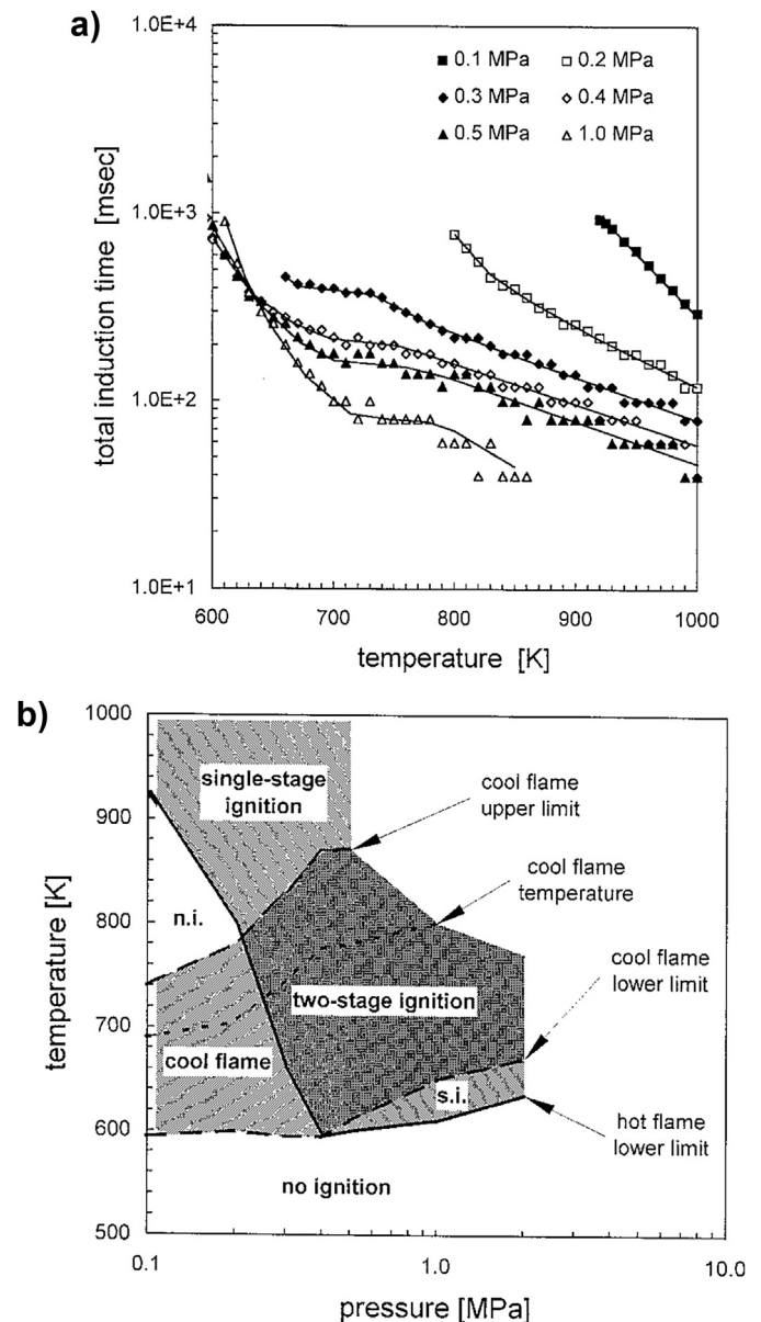
Fig. 26. (a) Total ignition delay (or induction time) versus ambient temperature at different pressures; (b) Various ignition regimes for the ignition of a n-heptane droplet with initial diameter of 0.7–0.75 mm.
