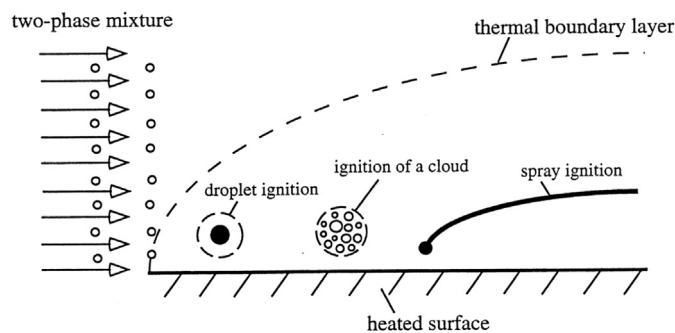
Fig. 1. A schematic of a two-phase mixture ignited in the thermal boundary layer of a heated surface. Three different ignition modes, namely, the droplet ignition, droplet cluster ignition, and spray ignition are illustrated. From Ref. [1].
